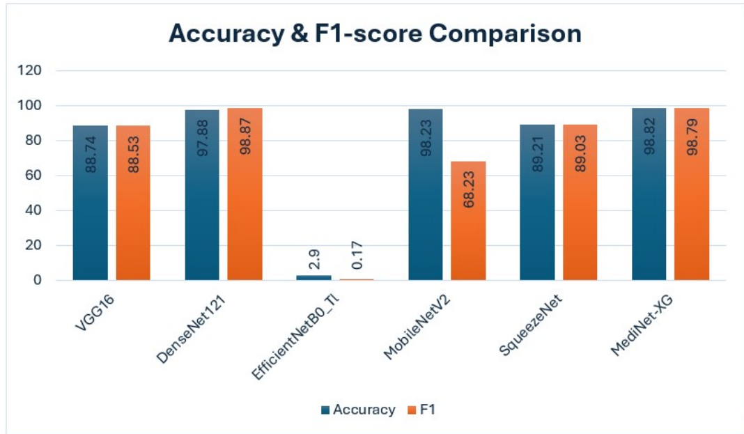
Figure 5.29: Accuracy comparison on prepared dataset[2].
