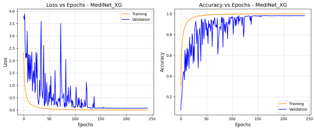
Figure 5.30: Aucc and Loss of MediNet-XG Model.
