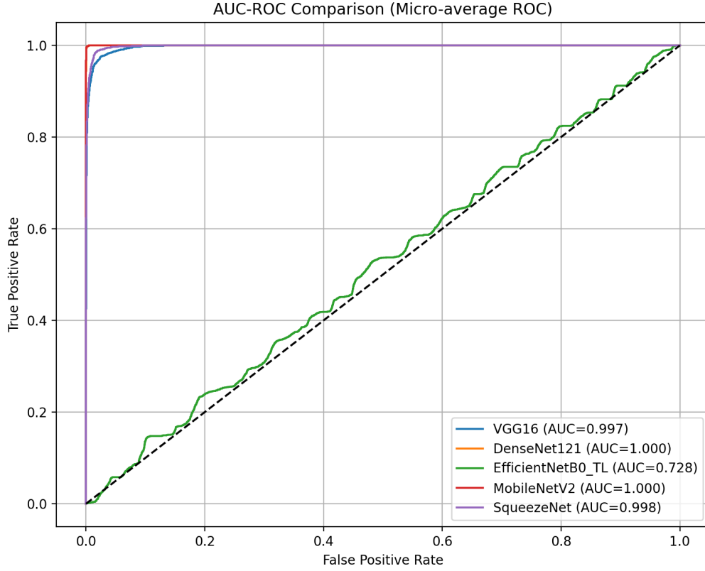
Figure 5.31: AUC-ROC comparison of various models.
