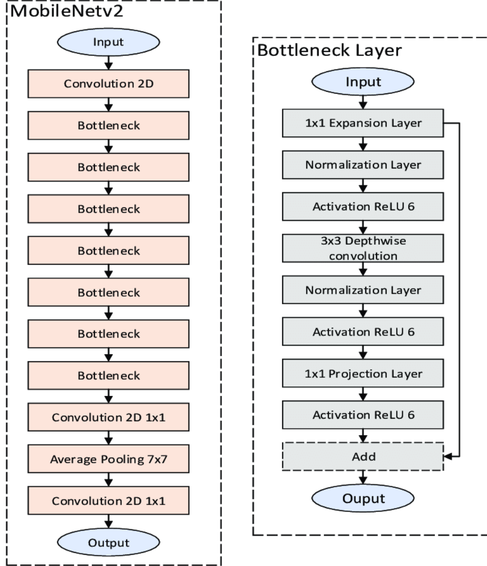
Figure 3.12: The MobileNetV2 architecture [28].
